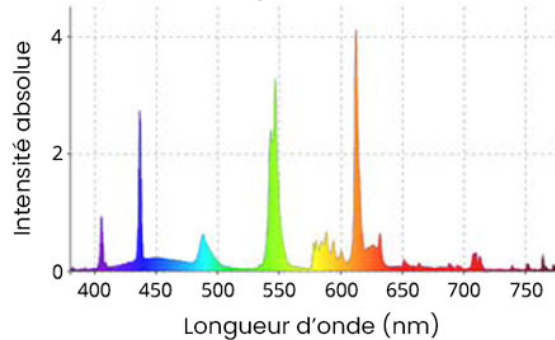
Spectre ampoule Fluo-compacte
