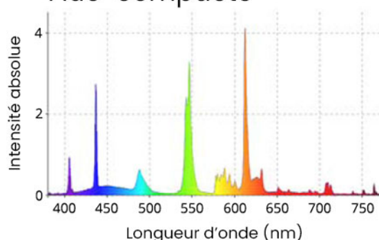
Spectre ampoule Fluo-compacte
