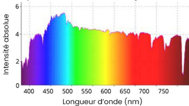
Spectre ampoule LED à filament
