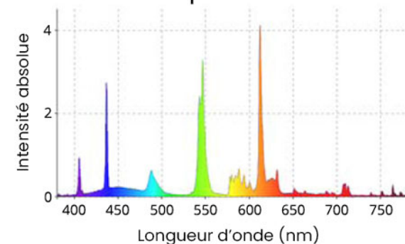
Spectre ampoule Fluo-compacte
