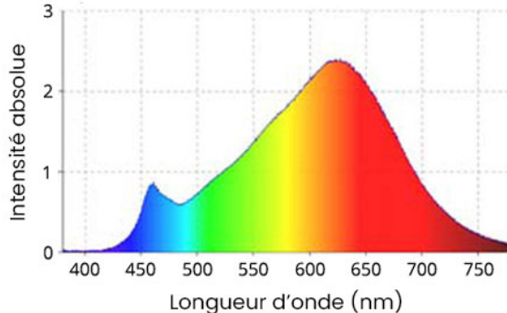
Spectre ampoule LED à filament
